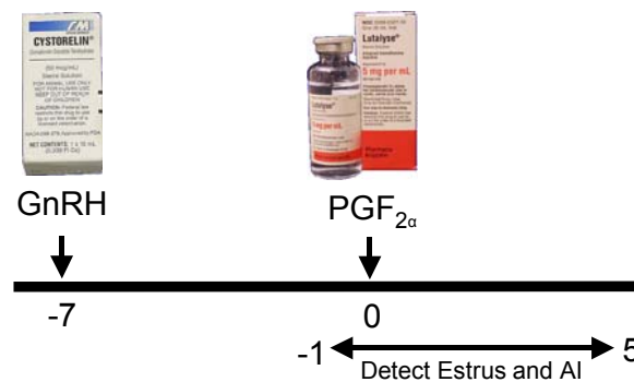
Figure 2. SelectSynch protocol
