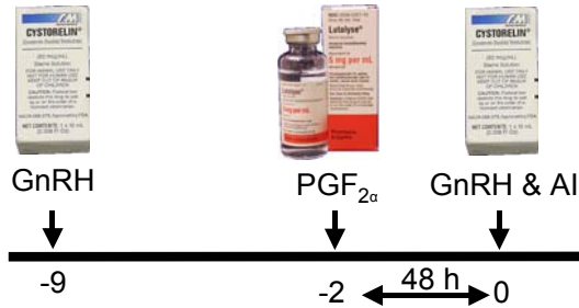
Figure 4. CO-Synch protocol
