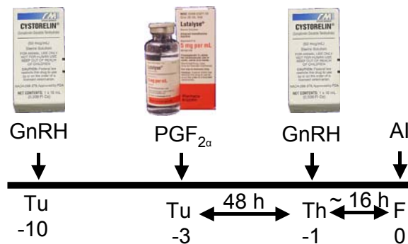
Figure 1. Ovsynch protocol
